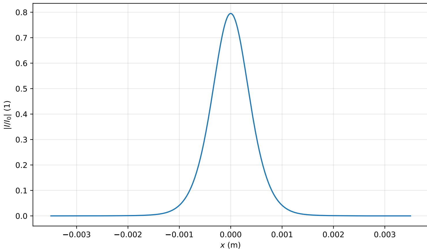
Intensity profile I(x, y = 0, z = 3.184m)/I_0 , P_{in}=0.7P_{cr} , artificial time
